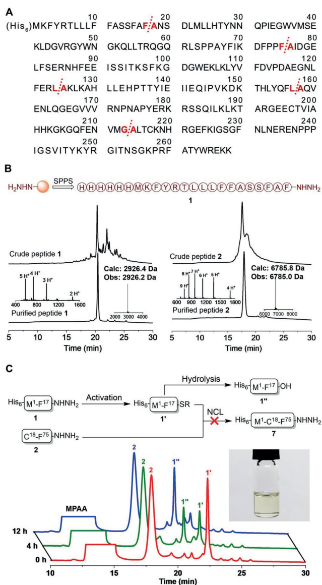
Figure 1. A) The amino acid sequence of His 6 -Hin-Lig. The full-length protein is divided into six segments (shown by dashed lines) and the ligation sites are highlighted in bold. B) Synthesis of peptide 1 by SPPS; analytical HPLC chromatogram ( \lambda = 214 nm) and ESI-MS spectra (including deconvoluted spectra) of the crude and purified peptides 1 (left) and 2 (right). C) Analytical HPLC traces ( \lambda = 214 nm) for the ligation of 1 with 2 for 0, 4, and 12 h. Key: peptide thioester of 1 ( 1' ), hydrolyzed product of 1' ( 1'' ).
