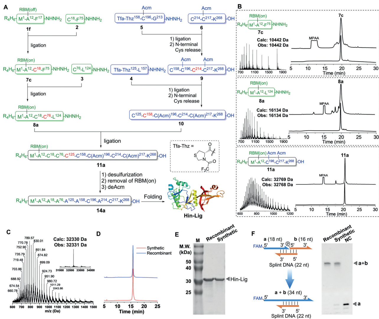
Figure 3. Chemical synthesis and characterizations of Hin-Lig. A) Synthetic route for Hin-Lig. B) Analytical HPLC traces of the ligations and the HPLC traces and ESI-MS spectra of the purified ligation products ( 7c , 8a , and 11a ; Supporting Information, Figures S18, S19, and S23). C) ESI-MS and deconvoluted spectra of synthetic Hin-Lig 14a . D) Analytical HPLC data of synthetic (red) and recombinant (blue) Hin-Lig. E) SDS-PAGE analysis of synthetic and recombinant Hin-Lig stained by Coomassie Brilliant Blue; protein marker (M). F) The DNA ligation assay of folded Hin-Lig and its analysis by PAGE in 8 M urea. The 5'-FAM-labeled DNA substrate a was ligated to the 5'-phosphate substrate b by recombinant and synthetic Hin-Lig; negative control with DNA substrates, ligase buffer, and refolding buffer, but without Hin-Lig (NC).
