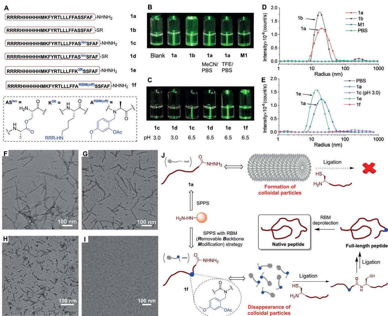
Figure 2. A) Amino acid sequences of peptide 1 and its modified analogues. B,C) The Tyndall effect of peptide 1 and its modified analogues. The tests were performed in the ligation buffer (0.1 M phosphate, 6 M Gn-HCl, pH 4.5) if not specially described; phosphate-buffered saline (PBS), acetonitrile (MeCN), 2,2,2-trifluoroethanol (TFE). D,E) Hydrodynamic radius distributions of blank, peptides 1a–1f , and M1 in the ligation buffer. F–I) TEM images of 1a (F), 1b (G), Arg 3 -tagged peptide 1e (H), and peptide 1f prepared by the RBM strategy (I). J) Principle of soluble but unreactive peptide and peptide ligation by the RBM strategy.
